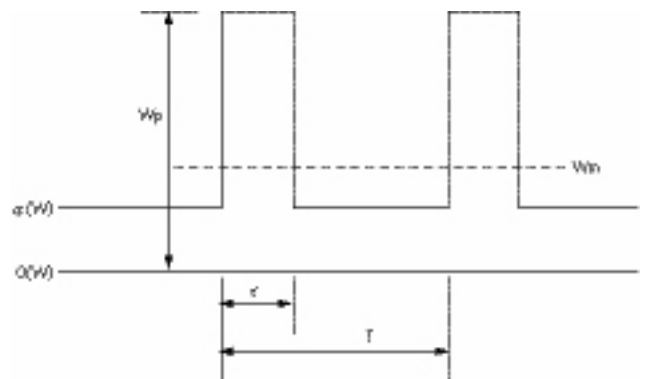
3. The drawing depicts a typical peak-output-power pulse waveform for a peak-rated supply where W_p is peak pulse power, W_m the maximum average output power, T the total period, t the pulse width during peak power, and \alpha the available non-peak power.
